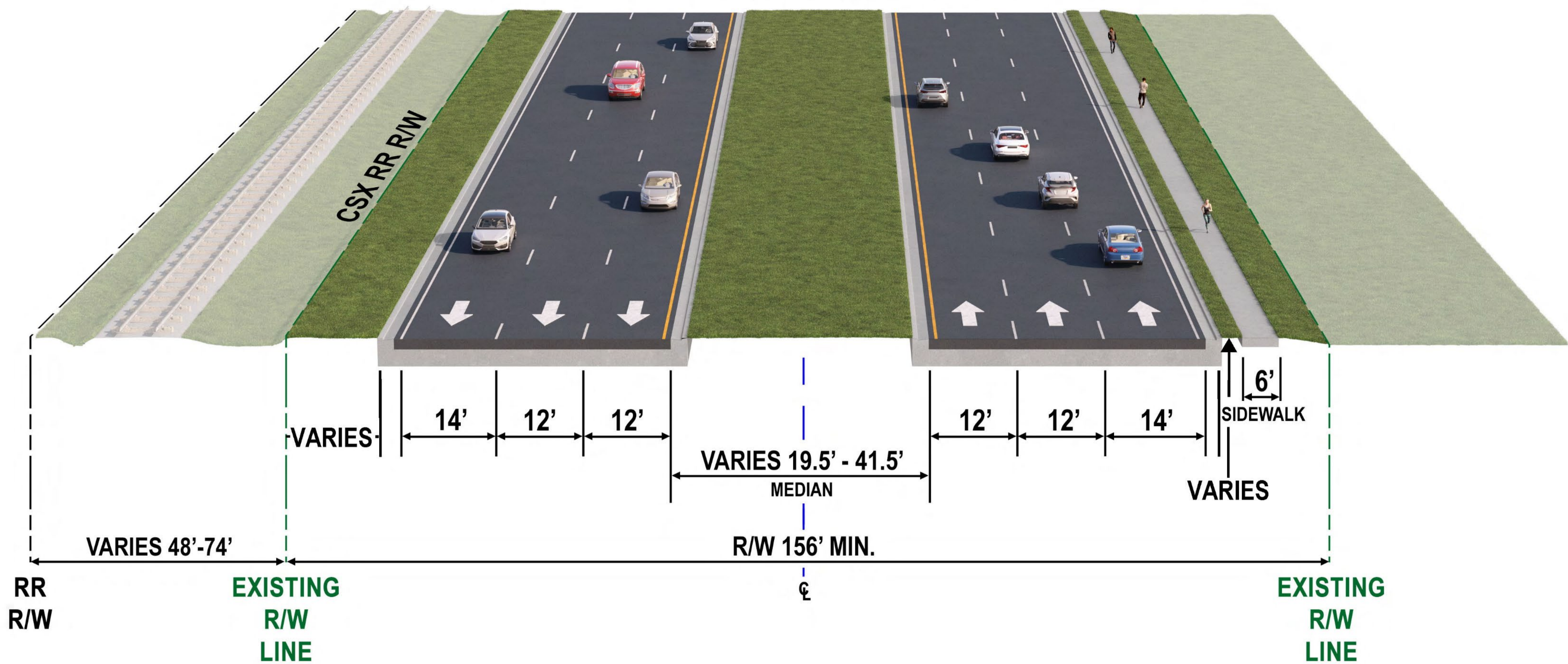
EXISTING ROADWAY TYPICAL SECTION – 6-LANE DIVIDED US 41 – LOOKING NORTH
