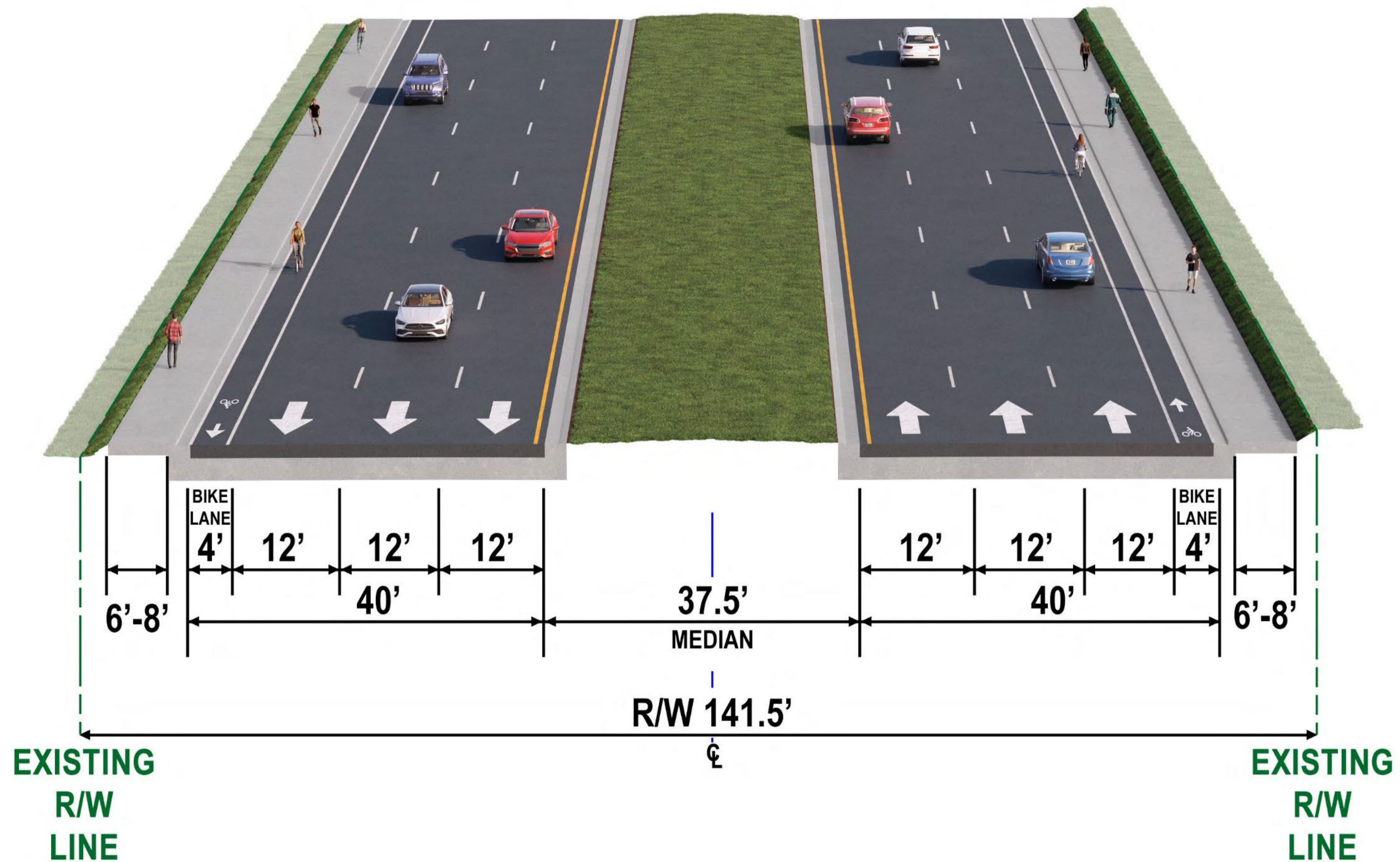
EXISTING ROADWAY TYPICAL SECTION – 6-LANE DIVIDED SR 54 – LOOKING EAST
