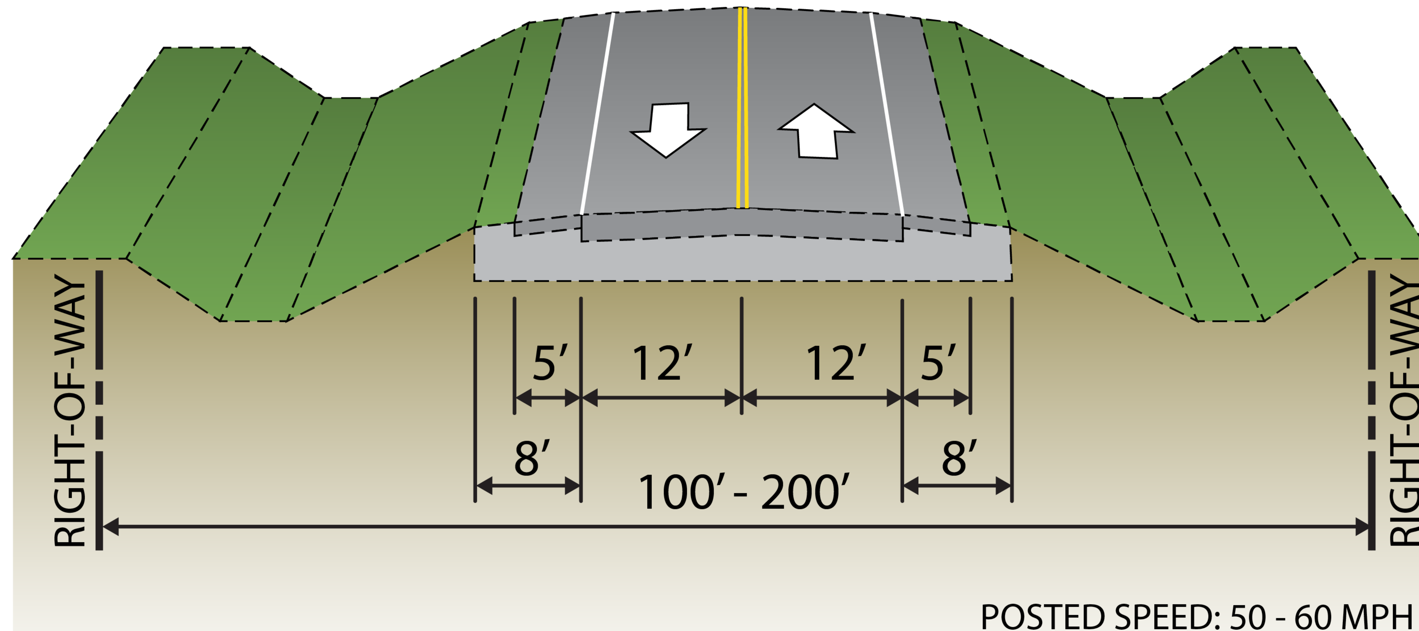
US 301 Existing Typical Section from Fowler Avenue to SR 56
